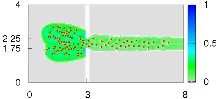
Figure 2: A mixed granular-diffuse crowd leaving a room through a door. This figure was kindly provided by the authors of [16].
